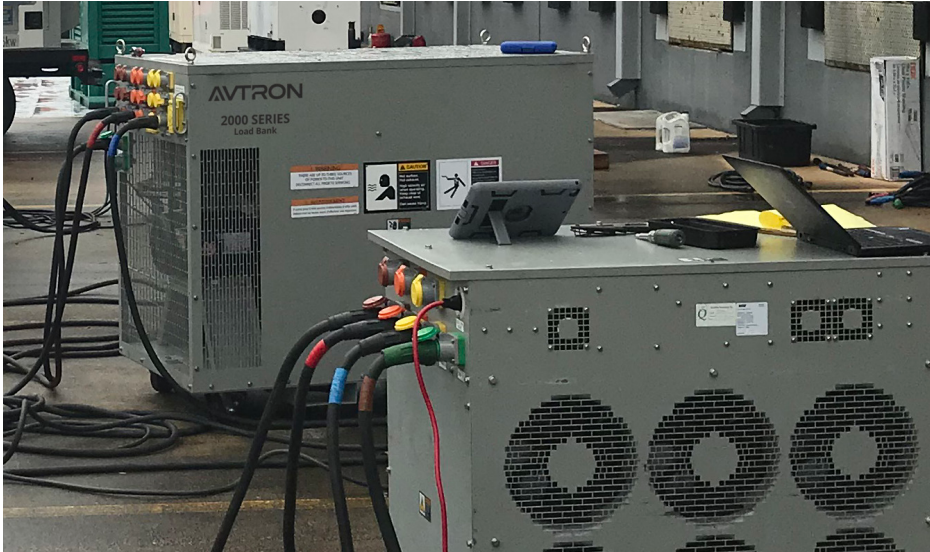
Load power cables shown connected on LC20 liquid cooled load bank shown above.
