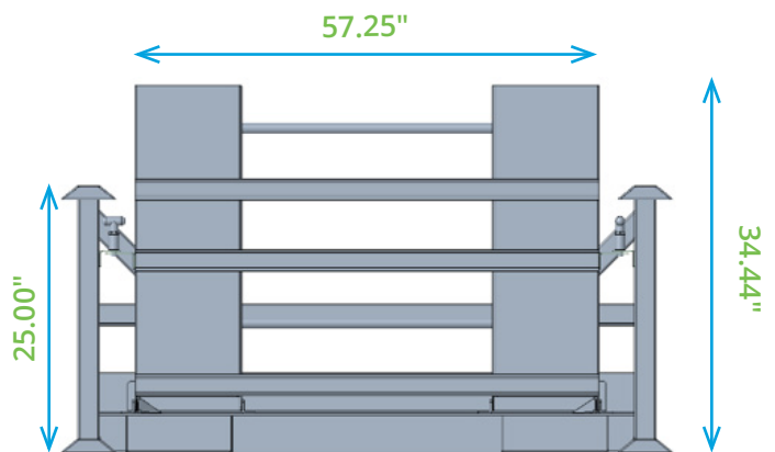
Image above: ramp in vertical position for load bank installation.
