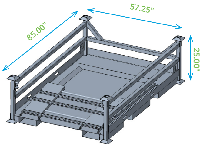
Image above: ramp folded inward without load bank.
